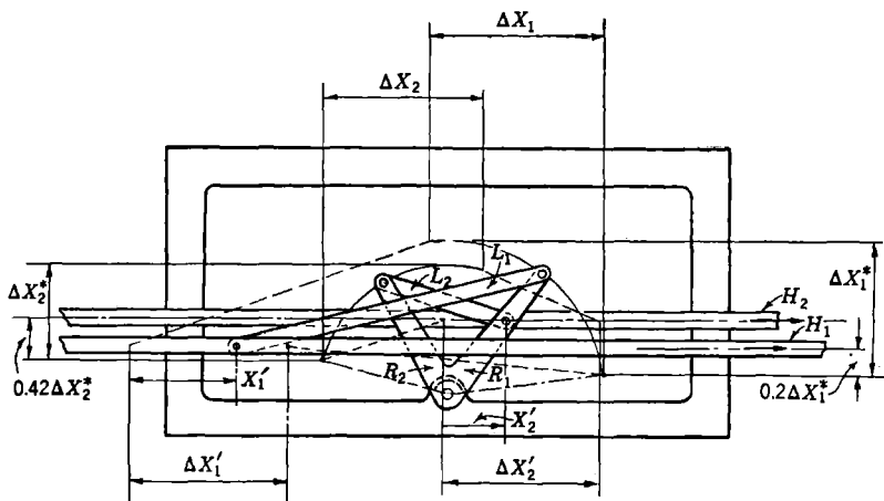
FIG. 4-26.—Nonideal double harmonic transformer generating, approximately, x_2 = \tan \alpha_1 , 0 < \alpha_1 < 70^\circ . Values of the constants are given in Eq. (80).
