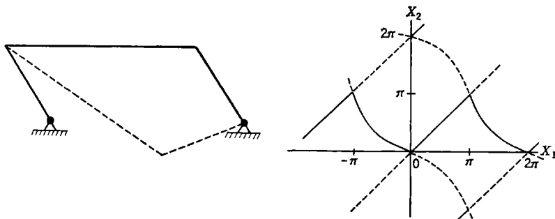
FIG. 5-6.—Three-bar linkage with B_1 = A_2 , A_1 = B_2 .
