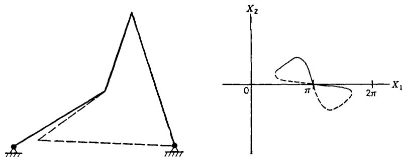
FIG. 5-5.—Three-bar linkage with A_1 - B_1 = A_2 - B_2 .
