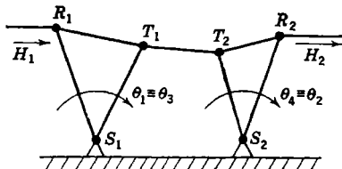
FIG. 6.1.—Three-bar linkage combined with two harmonic transformers.
