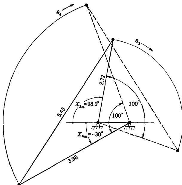
FIG. 6-12.—Mechanization of the tangent linkage: Fourth three-bar-linkage design.
