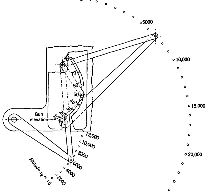
FIG. 10-4.—Schematic layout of ballistic computer.
