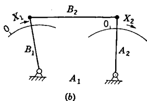
FIG. 7-1.—(a) Mechanization of a linear function. (b) Mechanization of an almost linear function.
