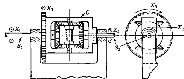
FIG. 1-1.—Bevel-gear differential.
