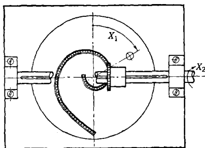
FIG. 1-20.—Pin gearing with pins on gear.
