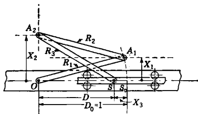
FIG. 2-13.—Elements of a bar-linkage multiplier.
