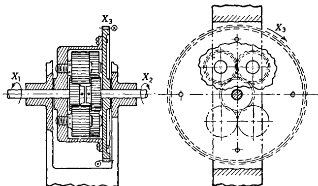
FIG. 1-2.—Cylindrical-gear differential.
