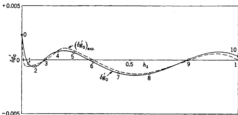
FIG. 7-4.—Gauging error in the first improved logarithmic linkage. Full line, result of exact computation. Dashed line, values expected on linear theory.
