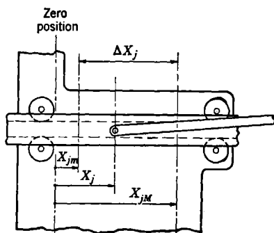
FIG. 3-2.—Slide terminal.
