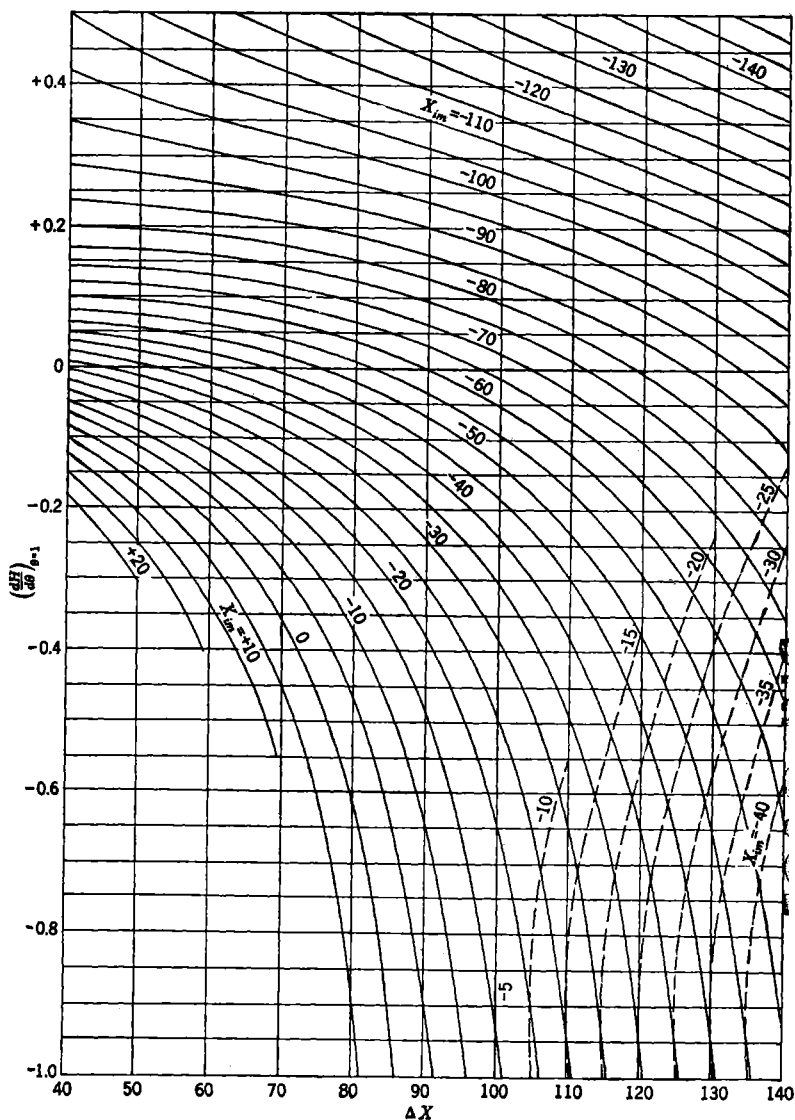
FIG. 4-18.—Logarithm of the final slope, (\frac{dH}{d\theta})_{\theta=1} , of ideal-harmonic-transformer functions, plotted against angular travel for a series of values of X_{im} . Dashed lines indicate that the final slope is negative.
