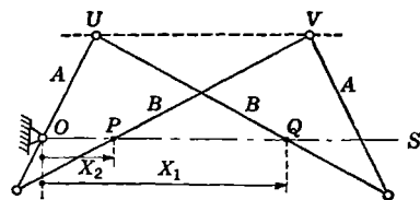
FIG. 2.5.—The Hart invisor.
