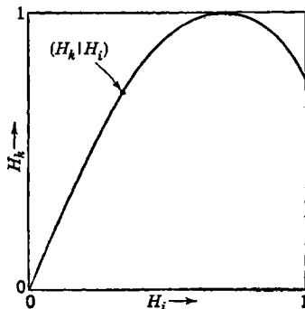
Fig. 3-6.—Graphical representation of a typical operator (H_k|H_i) .
