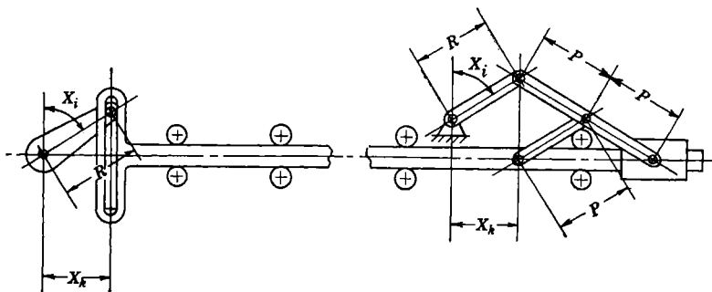
FIG. 4-1.—Ideal harmonic transformers.
