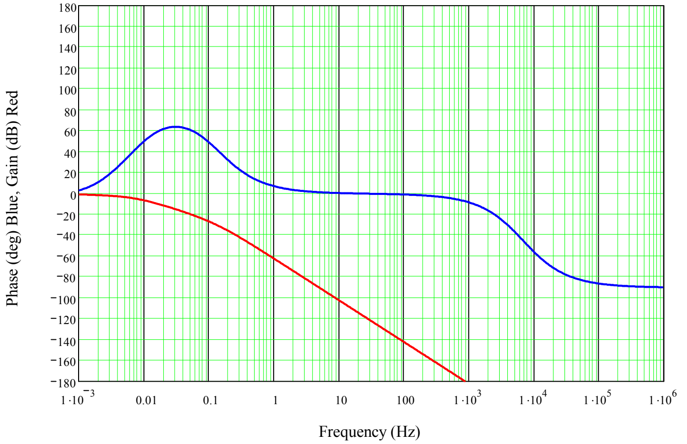
CW25 PLL - 10MHz transfer Function
